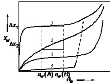
Figure: Four different materials exposed to a shift in water activity from a_w(A) to a_w(B) show different degree of water uptake \Delta x . The secant slope is a characteristic number of the material called water uptake potential w_p .
